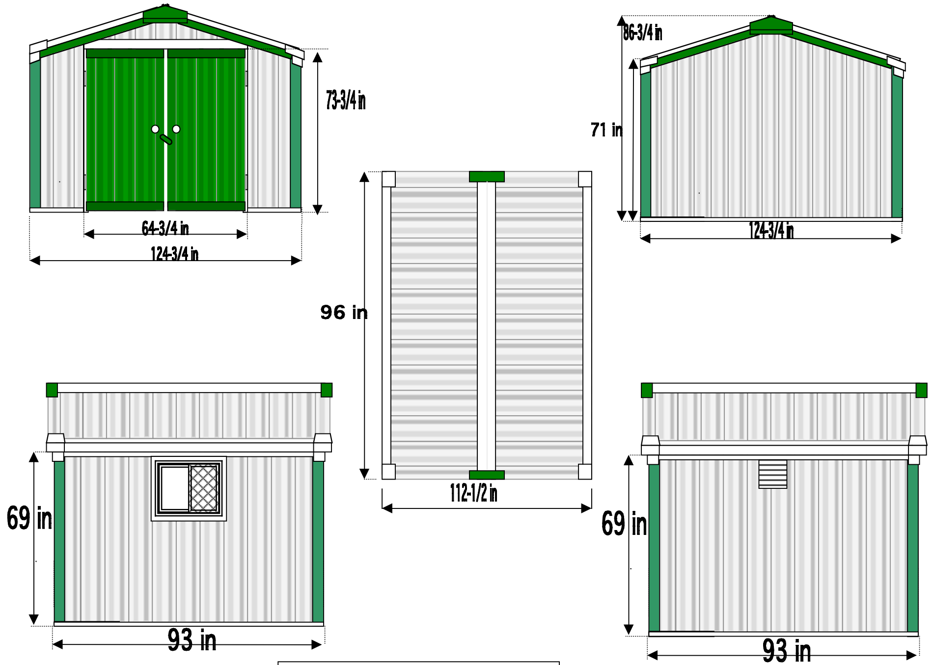
The side view of 10.5x8 Dan-Tec shed
